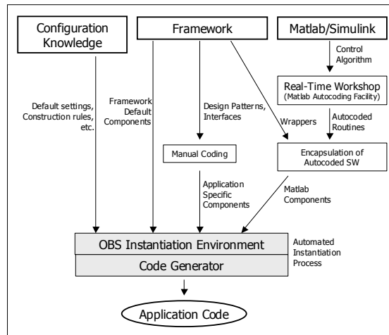
Fig. 2. Development process for embedded control software
