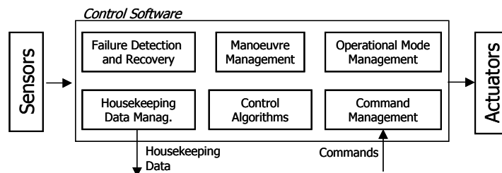
Fig. 1. Structure of typical control software
