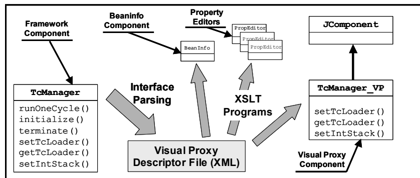
Fig. 4. Visual proxy generation process
